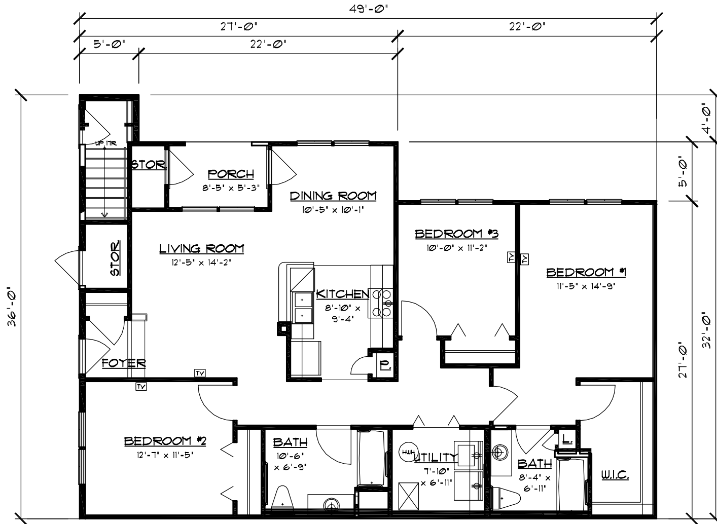
UNIT F FIRST FLOOR PLAN ANSI 1998 - TYPE A ACCESSIBLE GROSS AREA: 1,431 S.F. NET AREA: 1,375 S.F.
